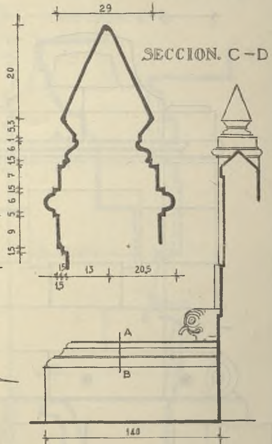
LATERAL
